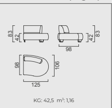
Midi Module (Right)
