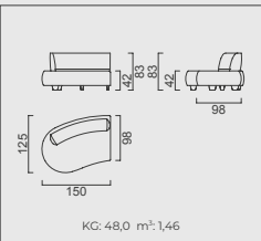
Curved Module (Left)
