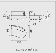
Curved Module (Right)
