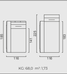
Relaxing Module (Left)
